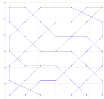
Figure 5-5: Left: Lissajous figure with a frequency ratio of 3:4 (left), Figure 5-6: Lissajous figure adapted to 7x7 measurement grid (right)
